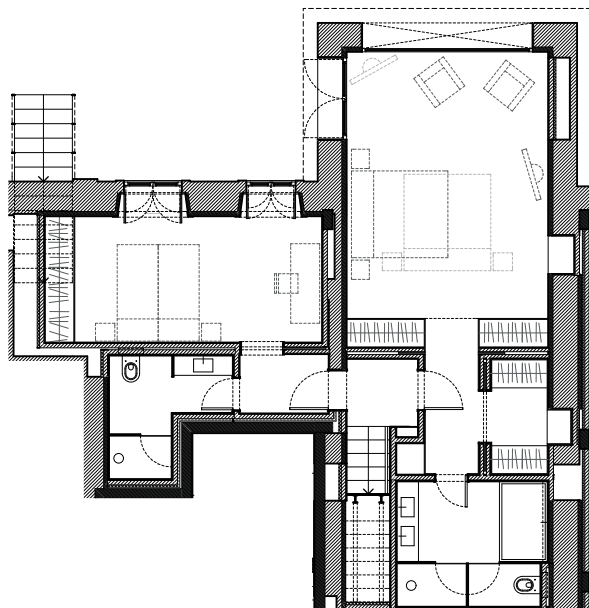
Piso -1 / Floor -1
